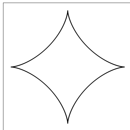
Figura 3.5: Astroide.
